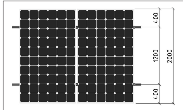
Portrait panel orientation 300W
