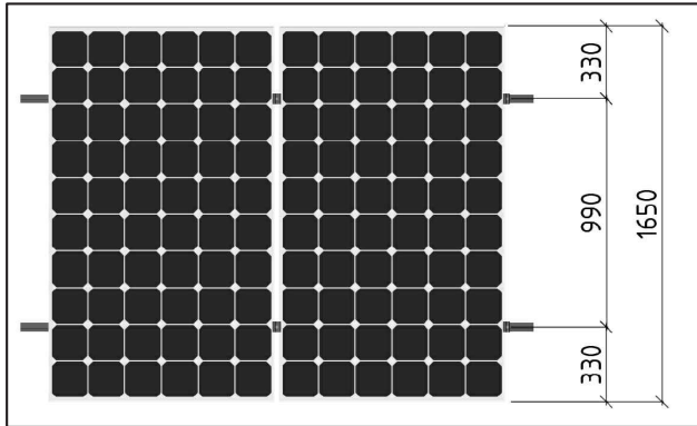
Portrait panel orientation 250W
