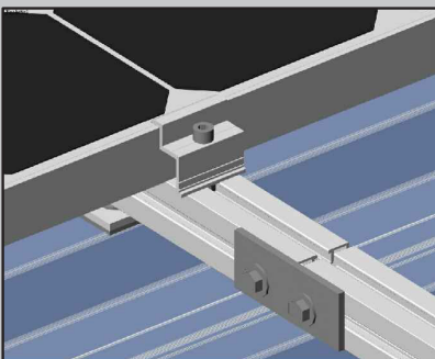
Join plate connection
